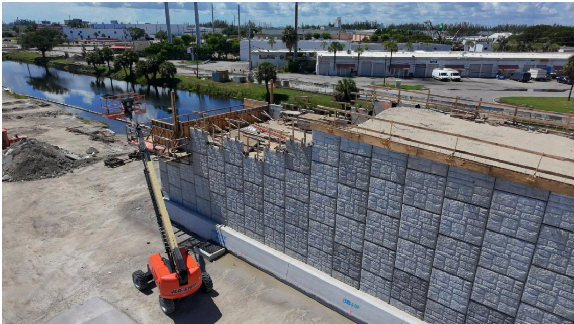
MSE WALL ALONG THE MIAMI CANAL
