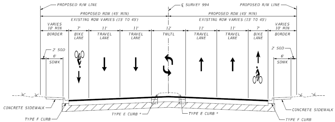
Figure 4-4 Four-Lane Road with TWLTL and On-Street Bicycle Lane
