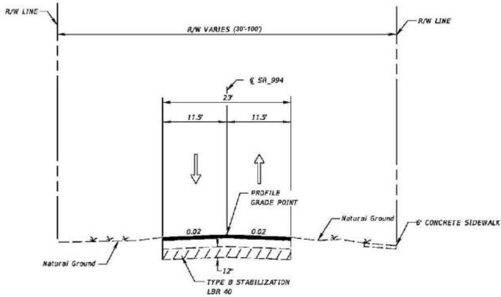
Figure 2-2 Existing Typical Section SR-994 from SW 137 Ave to SW 127 Ave
