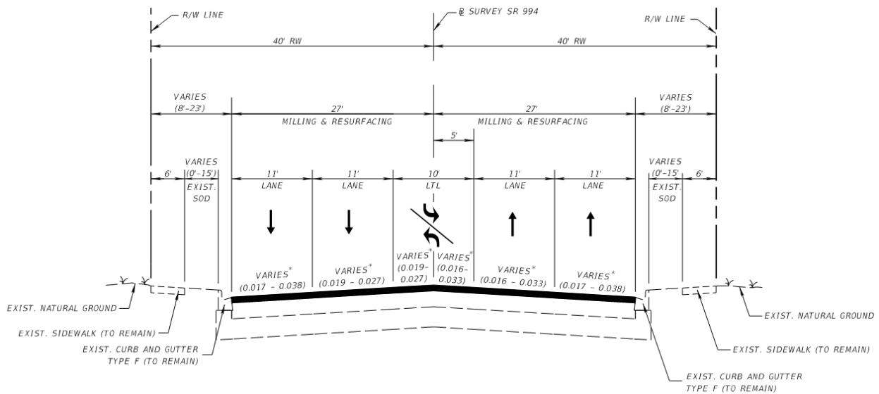
Figure 2-3 Existing Typical Section SR-994 from SW 127 Ave to SW 123 Place
