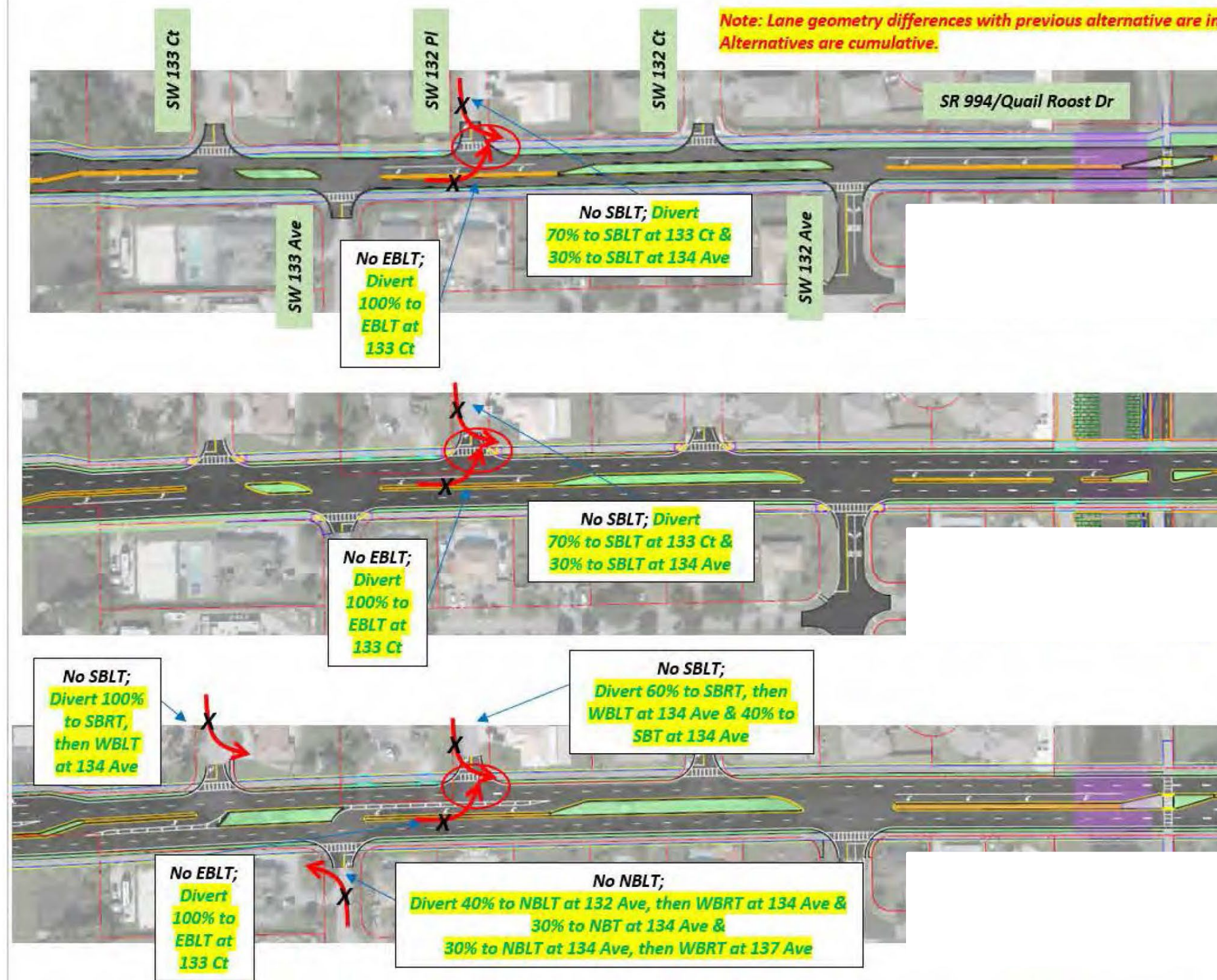
Figure 4-26 Traffic Diversion for SW 133 Ct, SW 133 Ave, and SW 132 Pl
