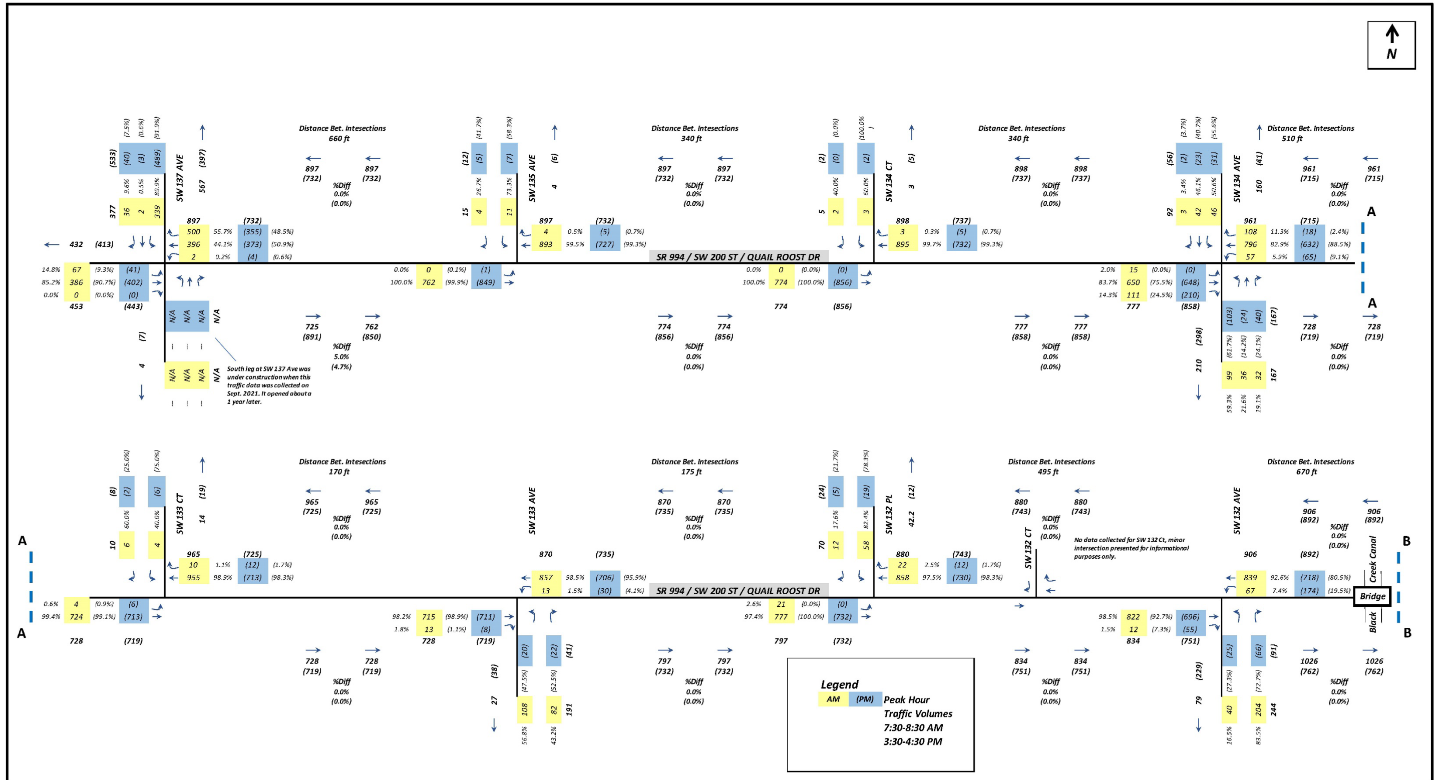
Figure 2-9 Existing AM & PM Peak-Hour Traffic Volumes (Balanced) – SW 137 Avenue to SW 132 Avenue
