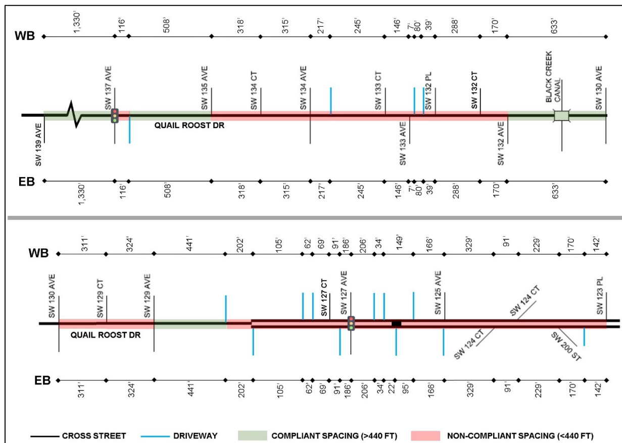
Figure 2-5 Existing Connection Spacings
