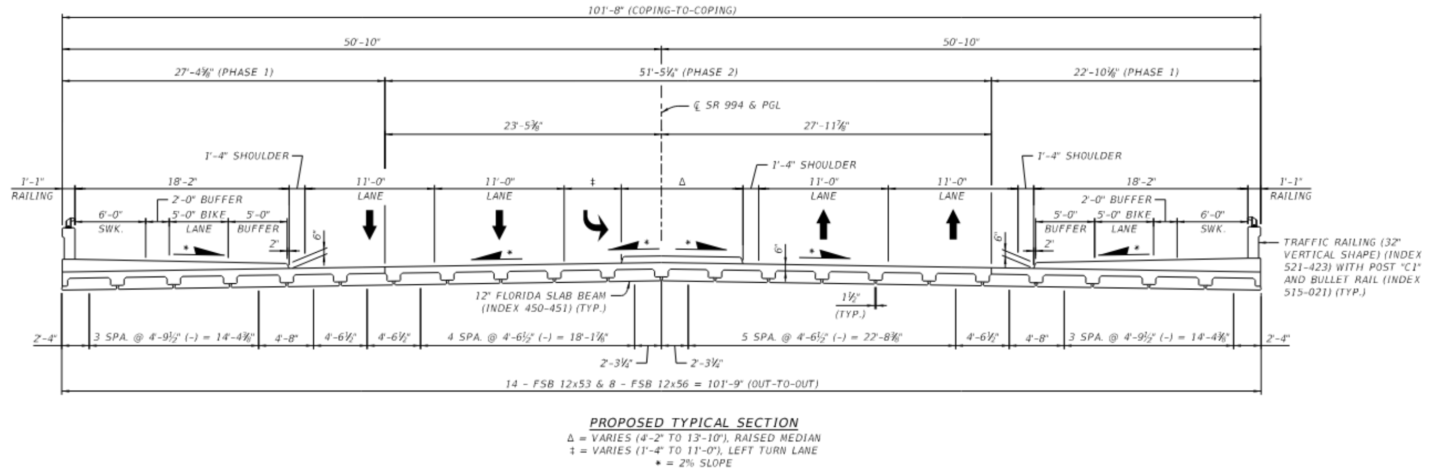
Figure 6-2 Proposed Bridge Typical Section
