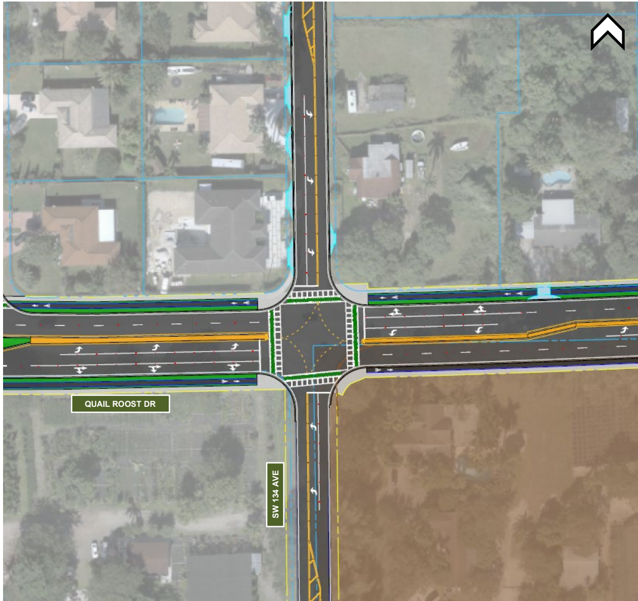
Figure 6-6 SR 994/Quail Roost Dr and SW 134 th Avenue Intersection
