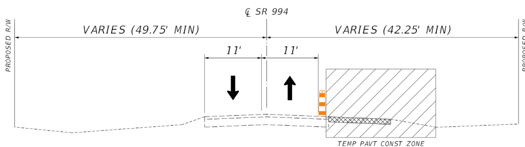
Figure 6-9 MOT Scheme 1 – Phase 1
