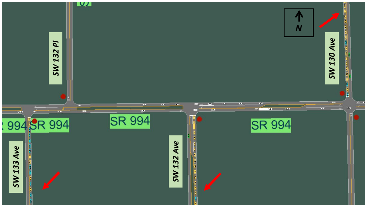
Figure 4-27 SimTraffic Vehicular Queues at Stop-Controlled Intersections
