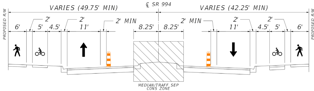
Figure 6-16 MOT Scheme 2 – Phase 4
