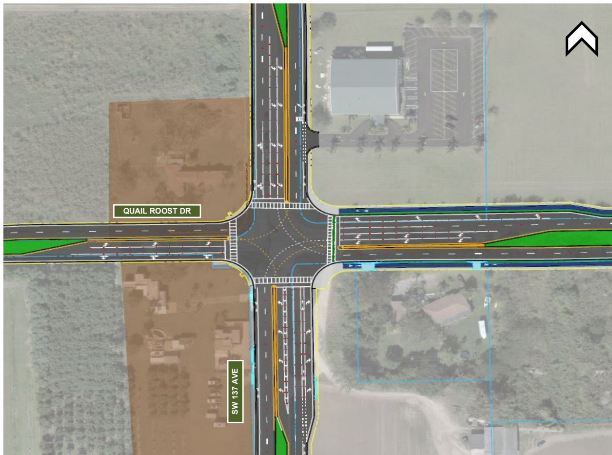
Figure 6-5 SR 994/Quail Roost Dr and SW 137 th Avenue Intersection
