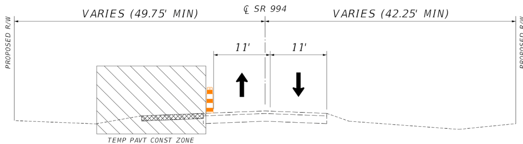
Figure 6-13 MOT Scheme 2 – Phase 1
