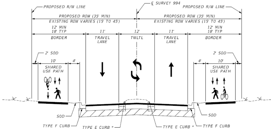
Figure 4-3 Two-Lane Road with TWLTL and Shared-Use Path
