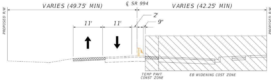
Figure 6-14 MOT Scheme 2 – Phase 2
