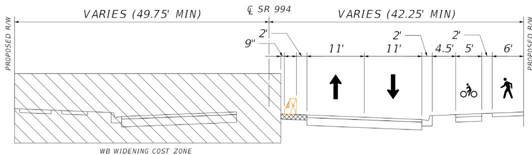
Figure 6-15 MOT Scheme 2 – Phase 3
