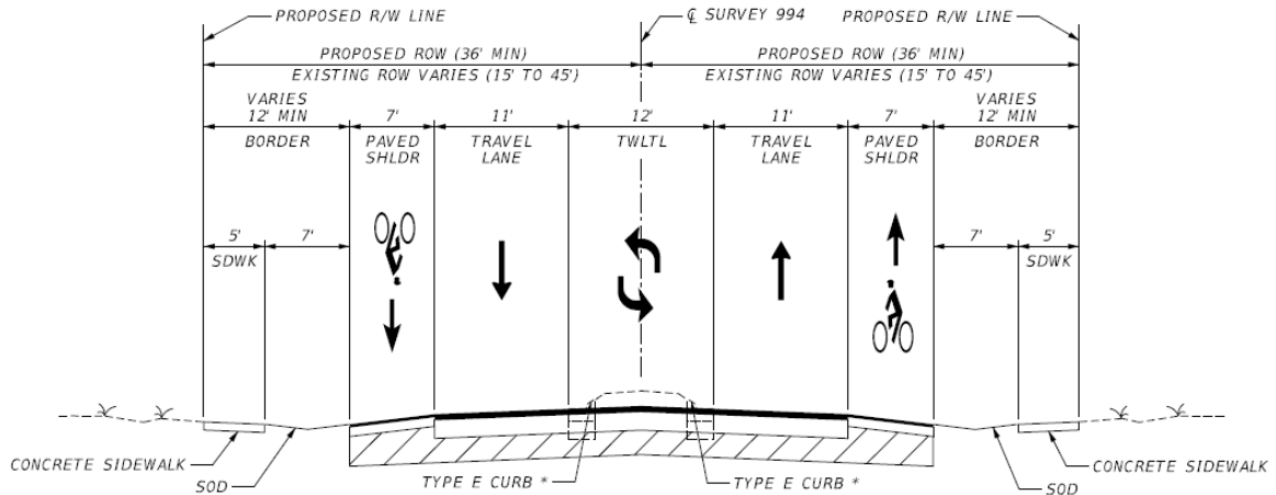
Figure 4-2 Two-Lane Road with TWLTL and Paved Shoulders
