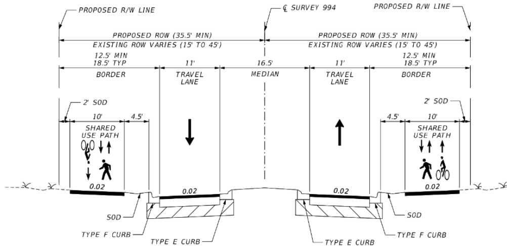
Figure 4-7 Two-Lane Road with 16.5-ft Median and Shared-Use Path
