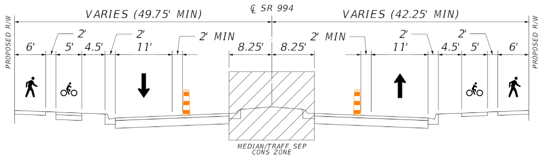
Figure 6-12 MOT Scheme 1 – Phase 4
