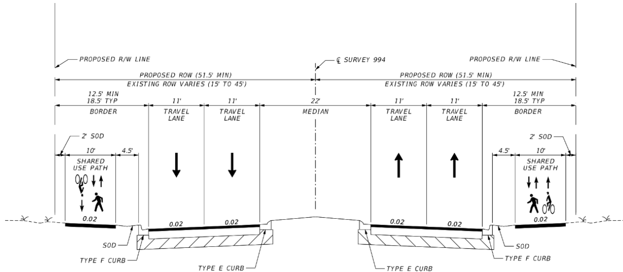
Figure 4-9 Four-Lane Road with Full-Width Median and Shared-Use Path
