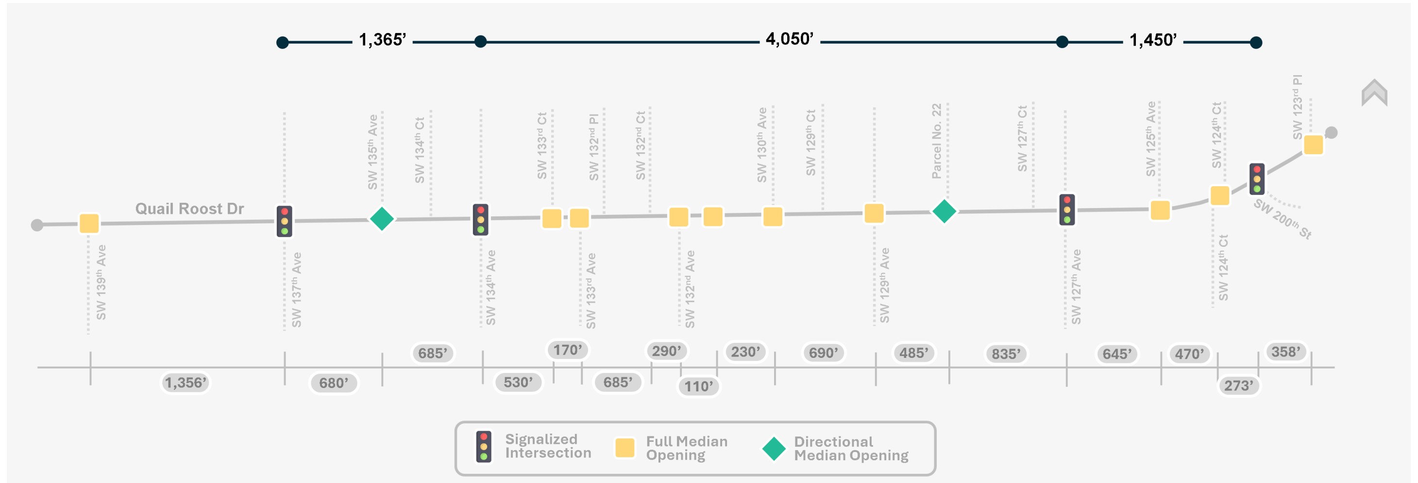
Figure 6-4 Preferred Alternative Median Opening Spacing
