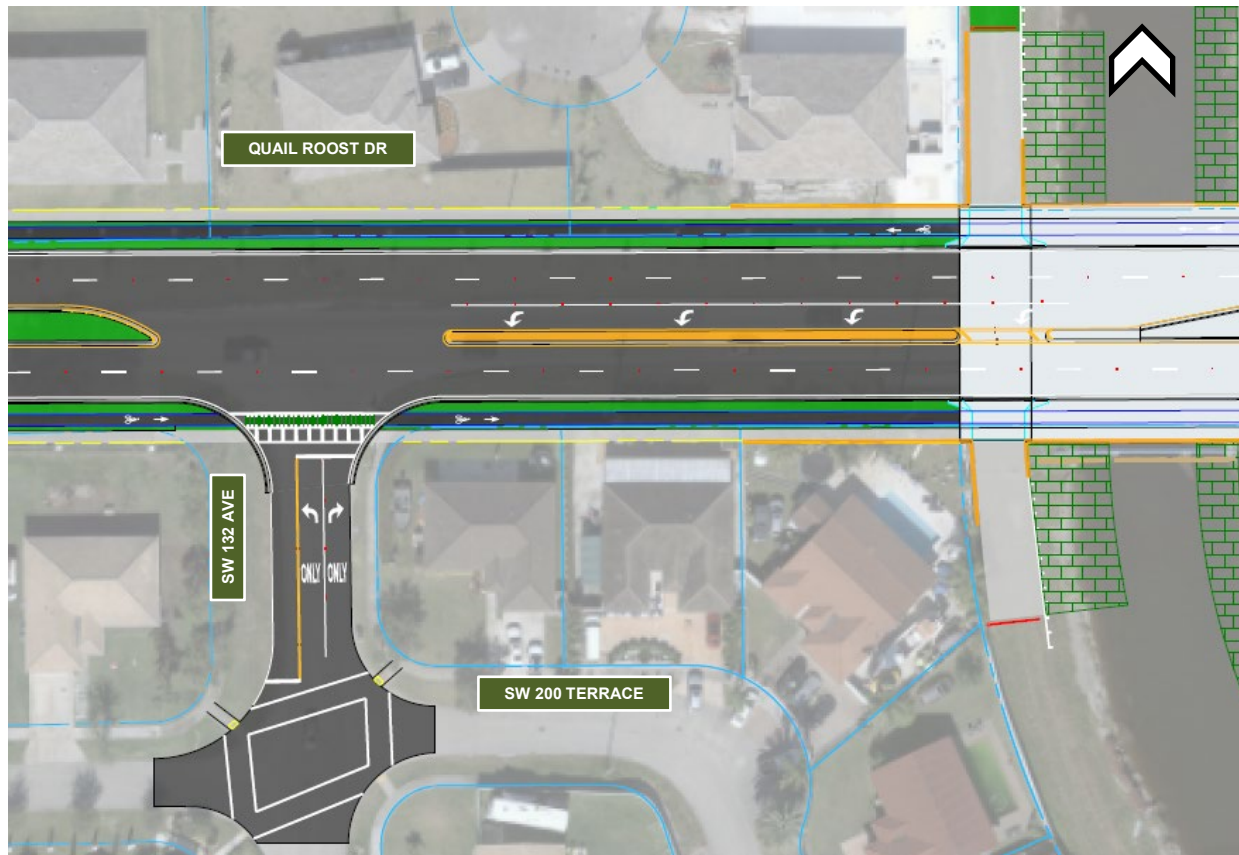
Figure 6-7 SR 994/Quail Roost Dr and SW 132 nd Avenue Intersection
