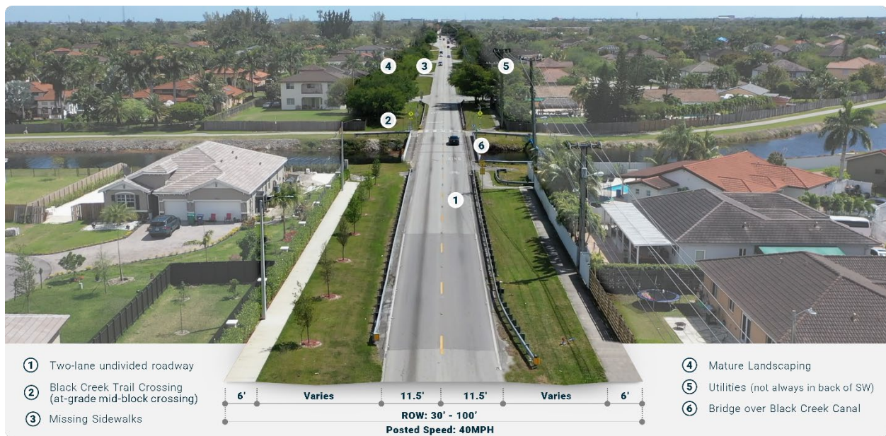
Figure 1-2 Existing Typical Section
