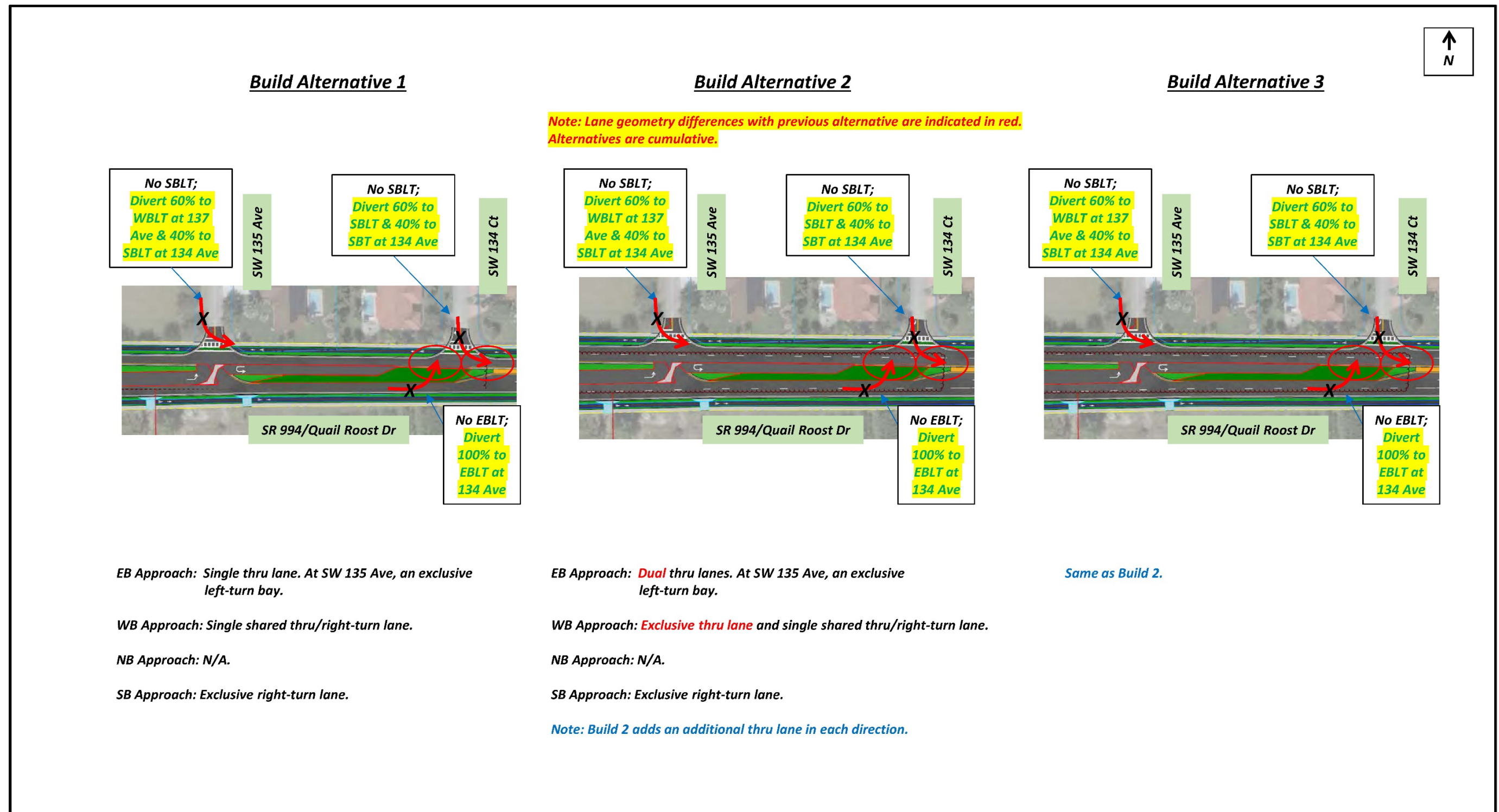
Figure 4-25 Traffic Diversion for SW 135 Ave and SW 134 Ct
