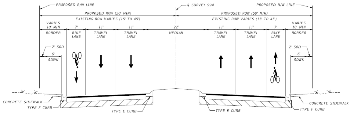
Figure 4-6 Four-Lane Road with Full-Width Median and On-Street Bicycle Lane
