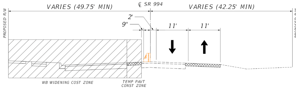
Figure 6-10 MOT Scheme 1 – Phase 2
