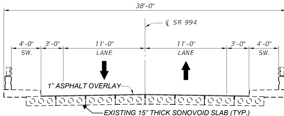
Figure 2-14 Existing Bridge Typical Section
