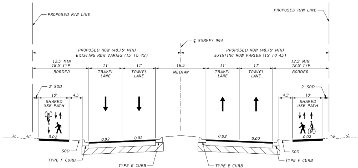
Figure 4-8 Four-Lane Road with 16.5-ft Median and Shared-Use Path
