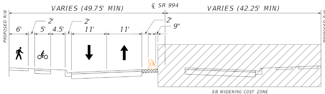
Figure 6-11 MOT Scheme 1 – Phase 3
