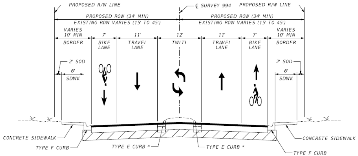
Figure 4-1 Two-Lane Road with TWLTL and On-Street Bicycle Lane
