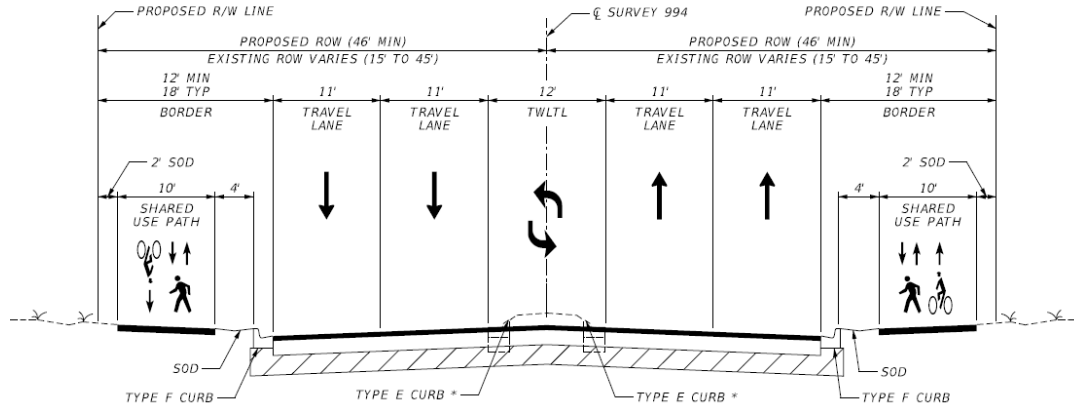
Figure 4-5 Four-Lane Road with TWLTL and Shared-Use Path
